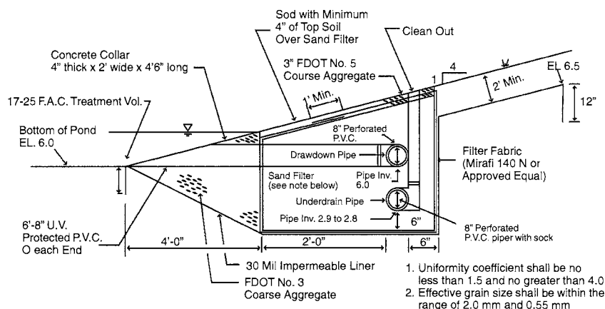
▲ Figure 2. Side view of detention pond with effluent filtration (Man-made underdrains).
