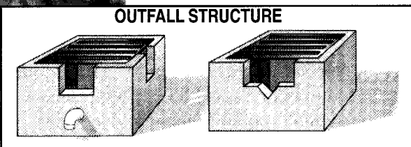
▲ Figure 3. Weir structure for wet detention pond. Alternative design could have a V-notch.
